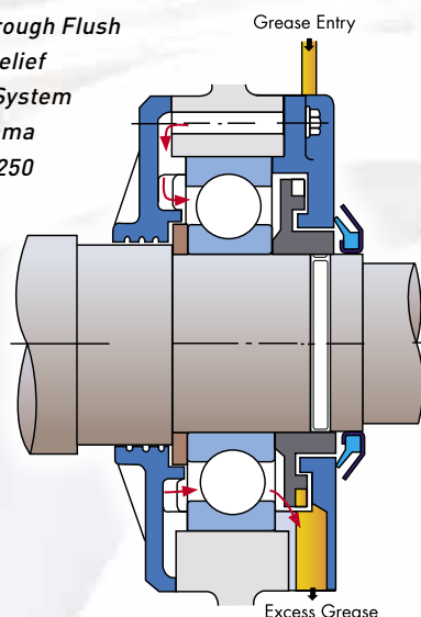
TECO Through Flush Grease Relief Bearing System with Brass Dust Flinger D280-315
